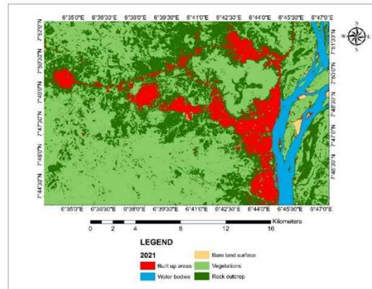
Figure 5: 2021 LULC Source: 2021 Landsat 9 OLI/TIRS imagery
